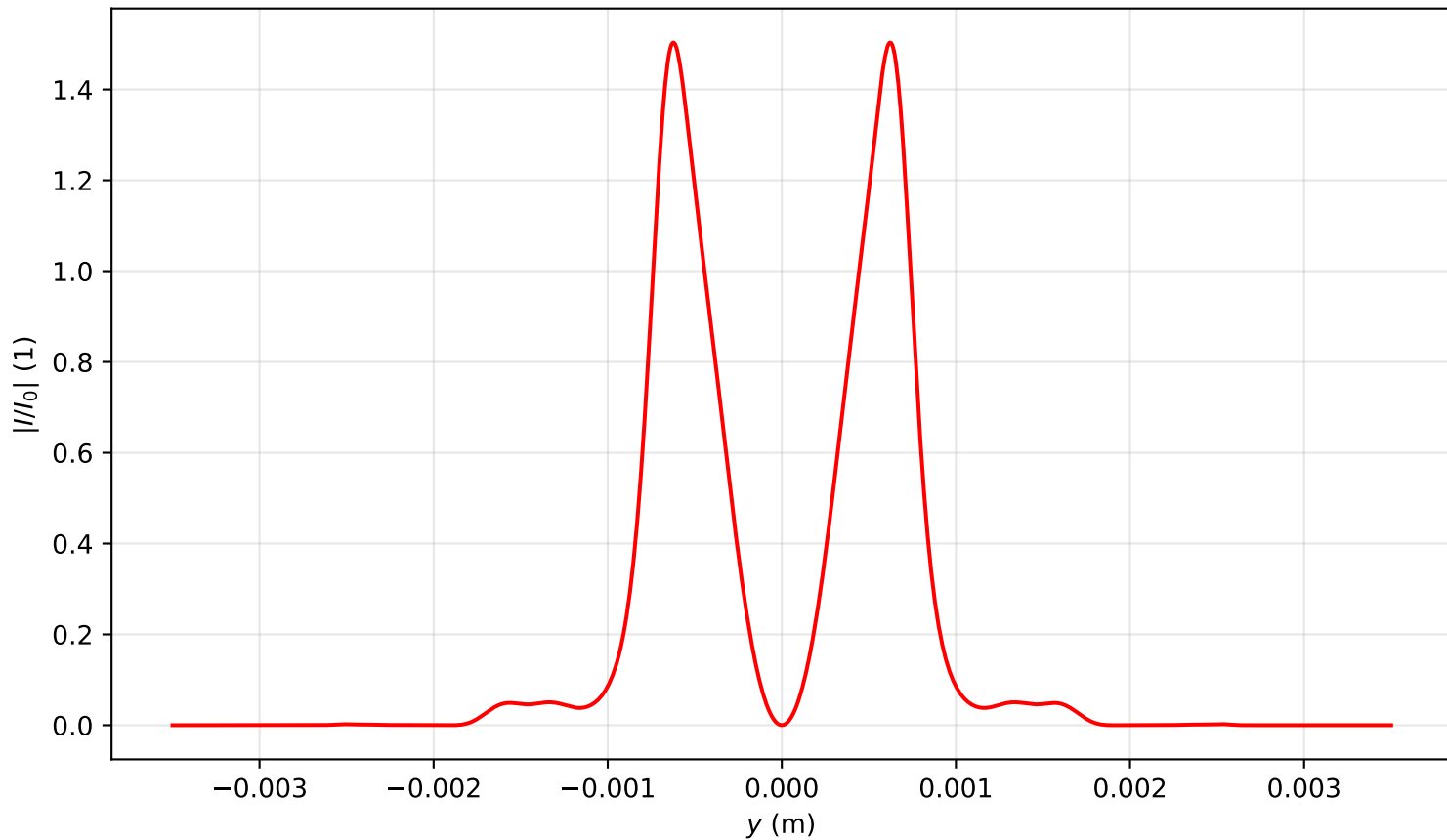
Intensity profile I(x=0, y, z=1.353)/I_0 , P_{in}=8.0P_{cr} , artificial time
